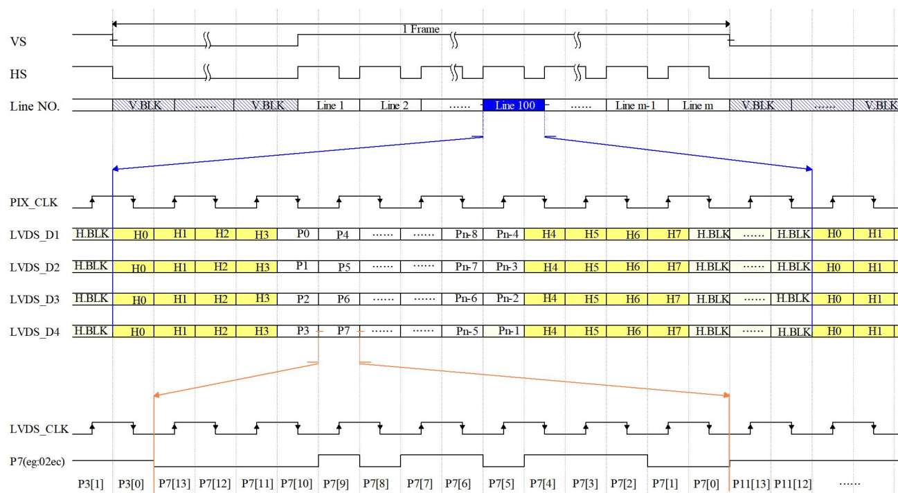
Figure 3.2 LVDS_H Digital Video Timing Diagram n \times m Array
