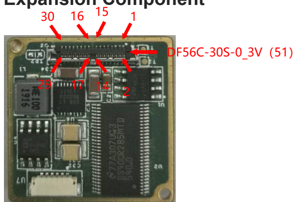
Figure 4.1 MR1100V100F008C Expansion Board
